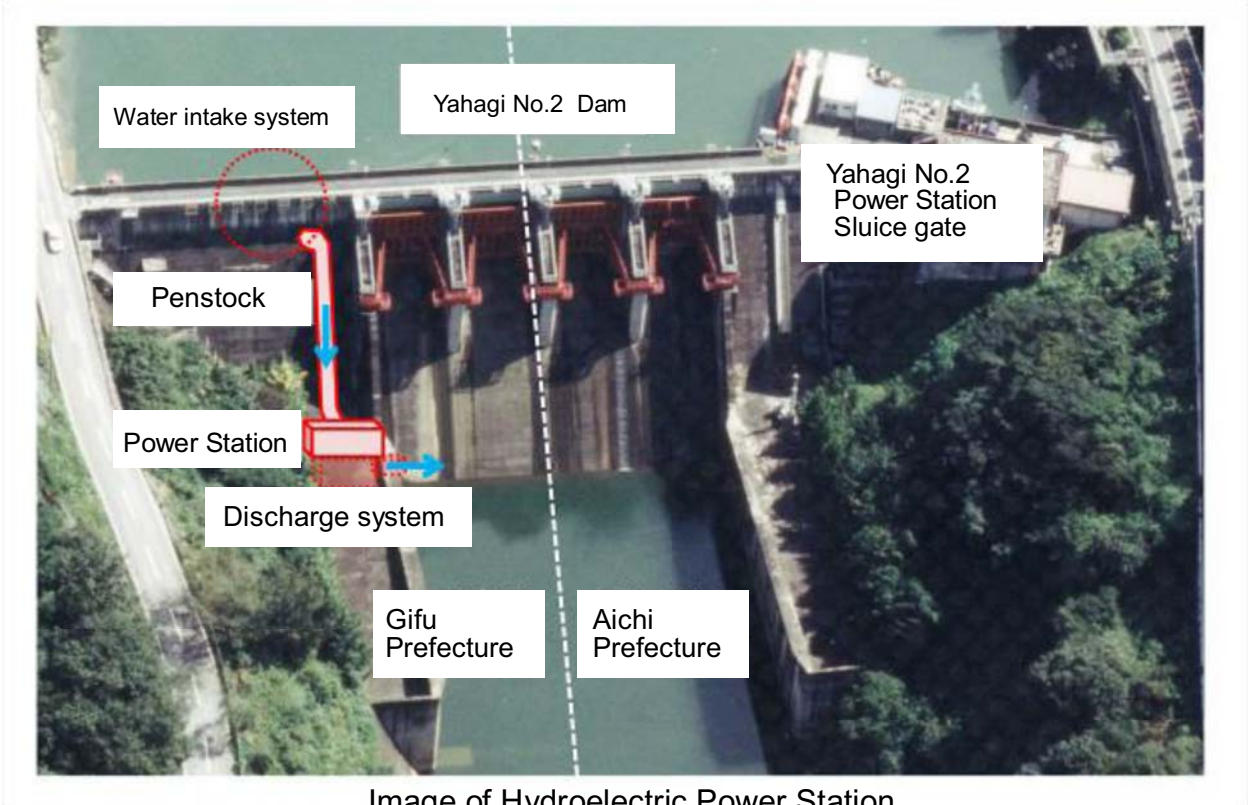
Image of Hydroelectric Power Station
