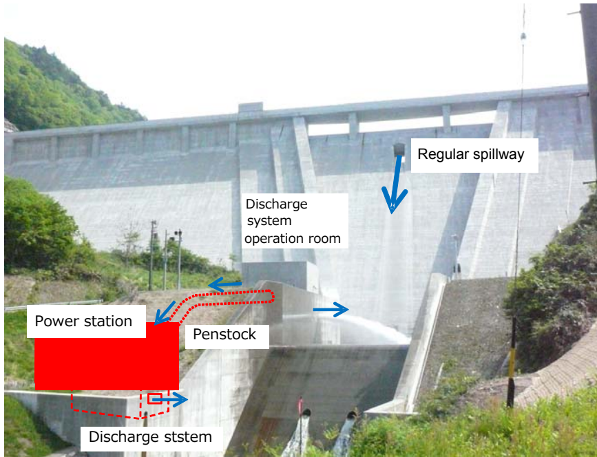
Image of Hydroelectric Power Station
