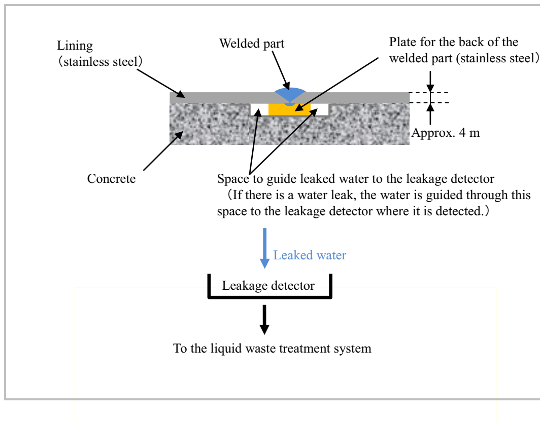
Condensate Tank Floor Image Diagram (side view)
