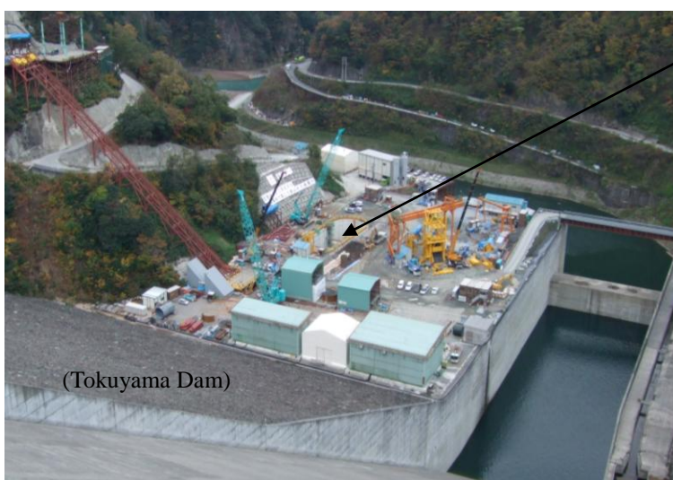
Construction status at Tokuyama Hydroelectric Power Station (November 16, 2011)
