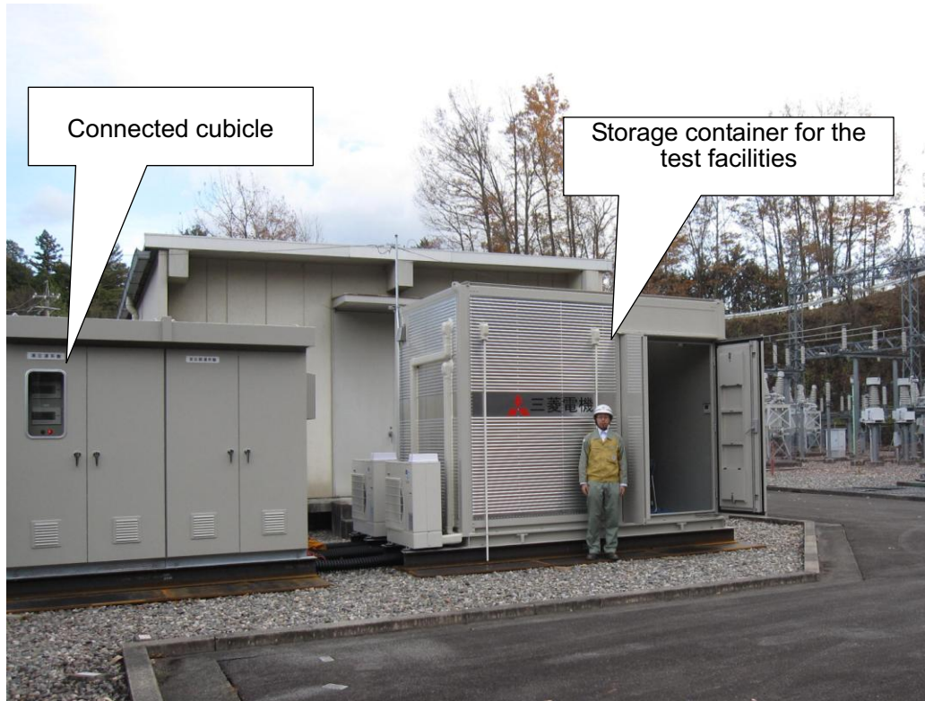
External Appearance of the Test Facilities
