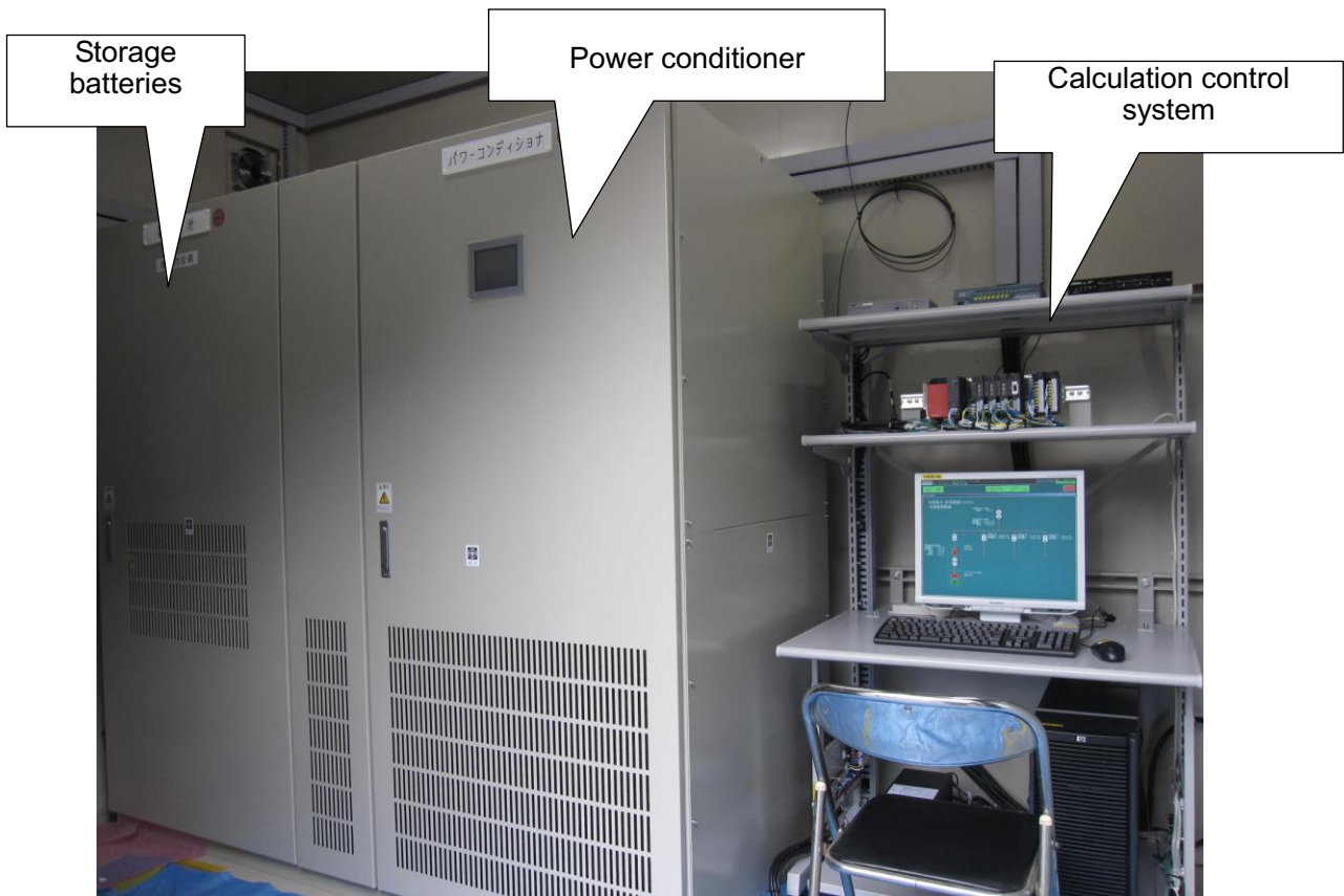
Inside the Storage Container for the Test Facilities
