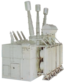
負荷時タップ切換変圧器 On-load tap-changing transformers (LRT)
